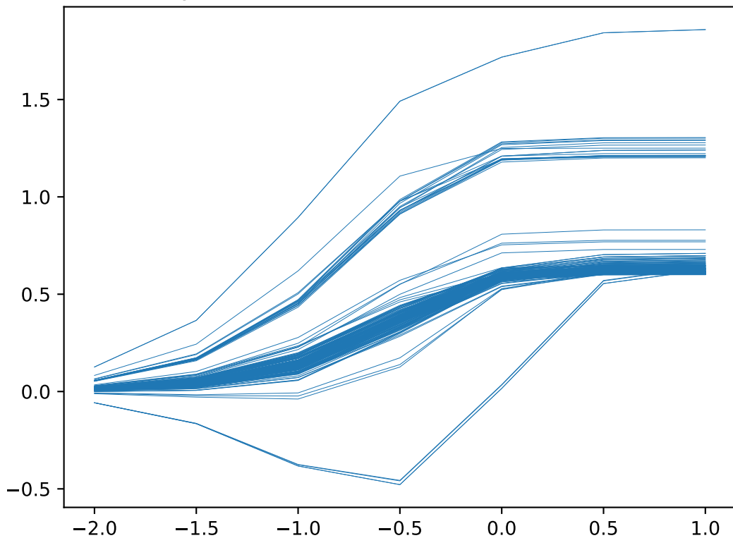
Dynamic Ricci Curvature for Geodesic 0.0
